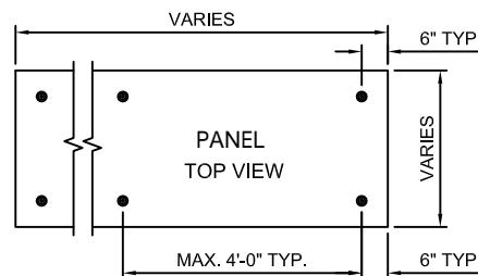
B WASHER PLATE DETAIL SP-02 SCALE: NA
