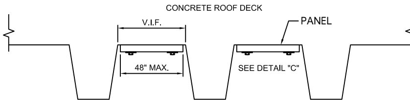
3 PANEL - TYP. ATTACHMENT DETAIL SP-02 SCALE: NA
