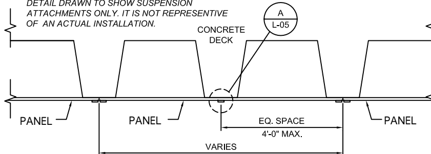
4 PANEL - TYP. ATTACHMENT DETAIL SP-02 SCALE: NA
