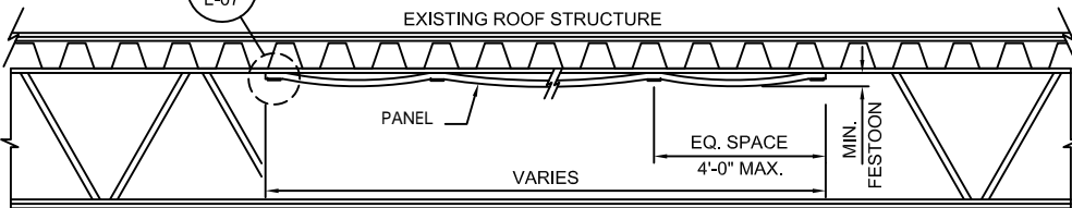
2 L-07 HORZ. - TYP. ATTACHMENT DETAIL SCALE: NA
