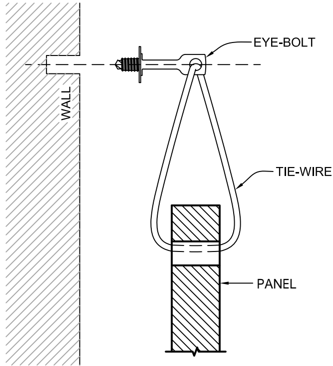
A ATTACHMENT DETAIL CL-08 SCALE: NA
