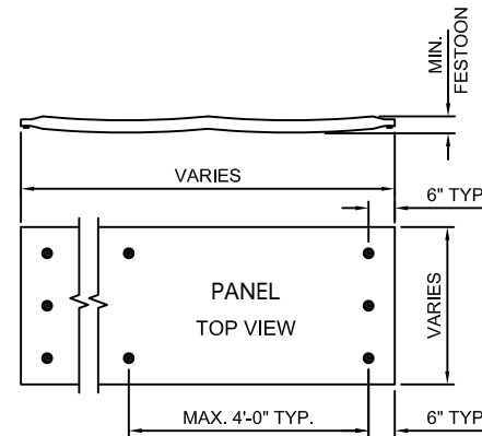
A L-07 HARDWARE ATTACHMENT DETAIL SCALE: NA
