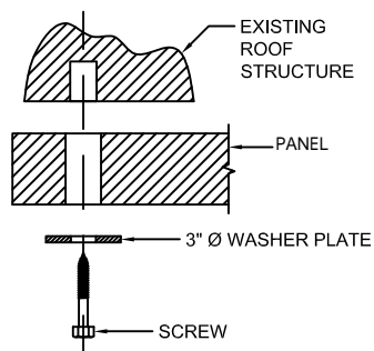
A HARDWARE ATTACHMENT DETAIL SP-02 SCALE: NA
