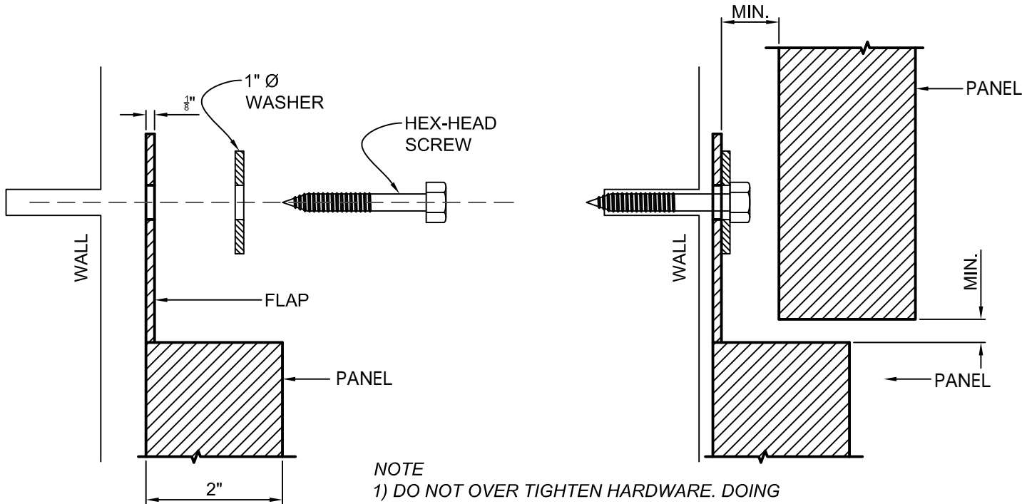
1 FRONT ELEVATION CL-08B SCALE: NA
