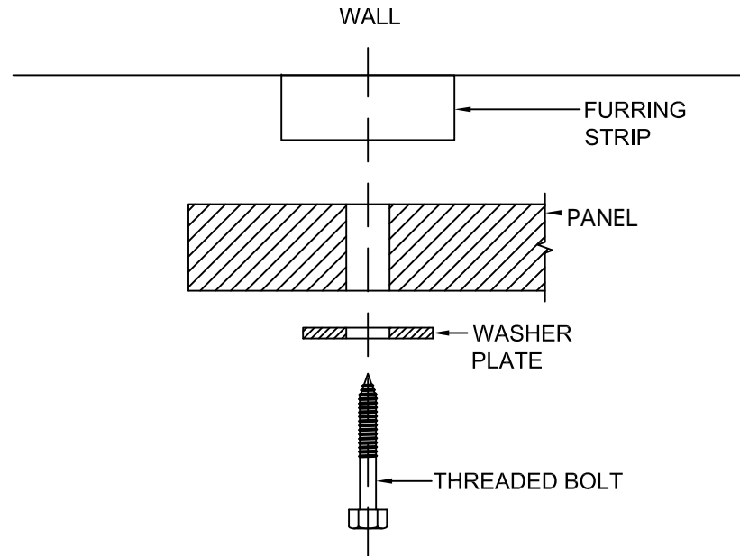
A ATTACHMENT DETAIL SP-04 SCALE: NA
