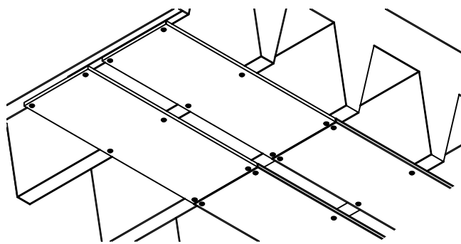
2 VIEW FROM BELOW SP-02 SCALE: NA
