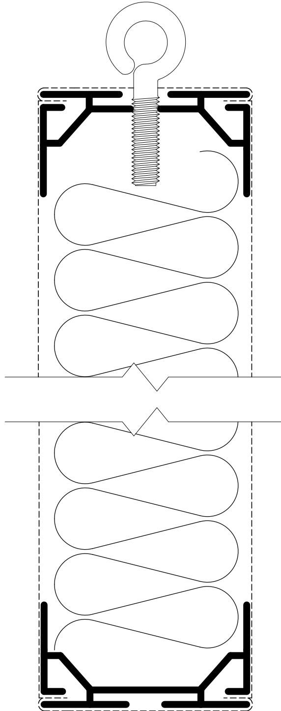
Baffle: 2-1/8" - Perimeter - Square - With Hanger Drawing Number: 17.1.00
