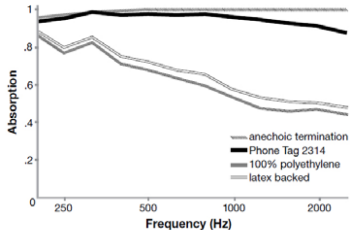
Acoustical Performance for Panel Applications (ISO 10534-2)
