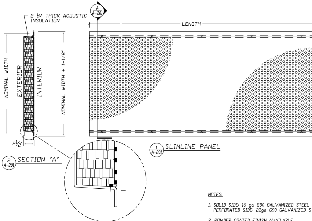
BARRIER PANEL 24" NOM. AND 18" NOM.
