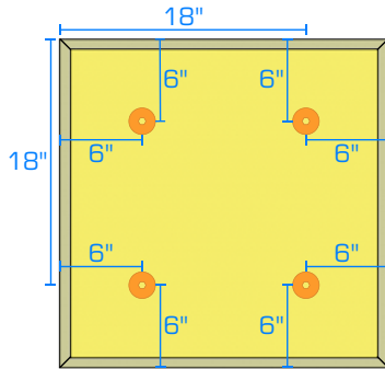
2' X 2' WALL PANEL
