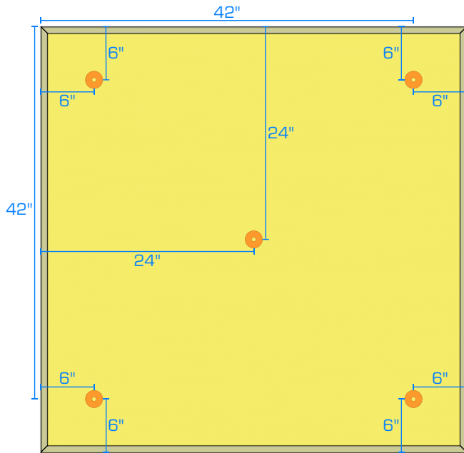
4' X 4' WALL PANEL
