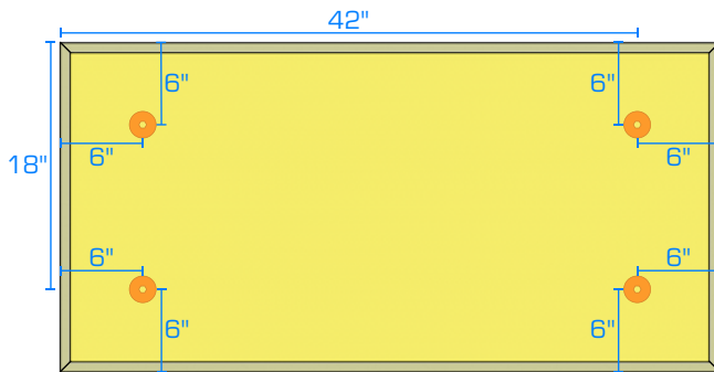
2' X 4' WALL PANEL
