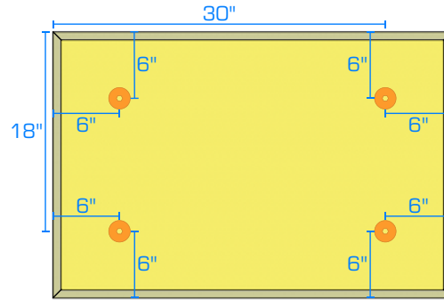
2' X 3' WALL PANEL
