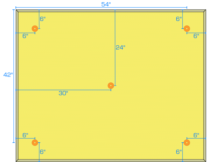
4' X 5' WALL PANEL
