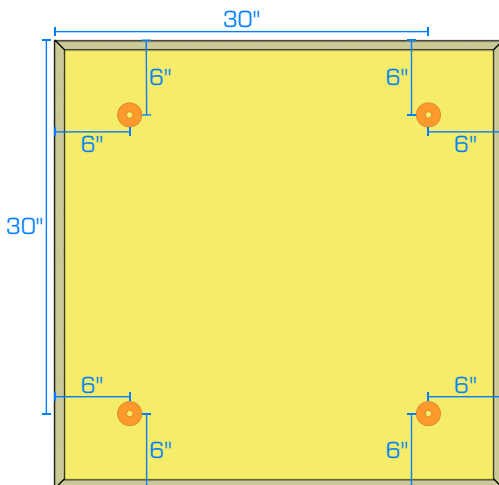
3' X 3' WALL PANEL
