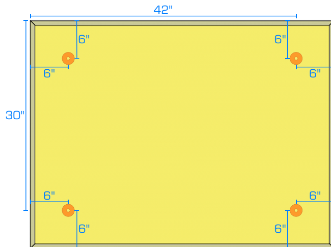
3' X 4' WALL PANEL
